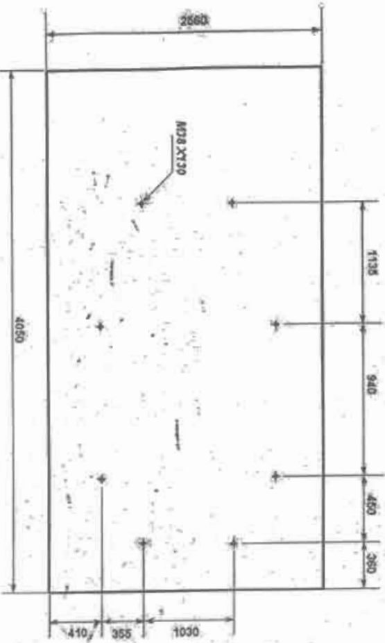
CONCRETE FOUNDATION TOP VIEW
